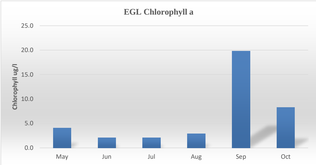
Figure 7 Chlorophyll Trend
